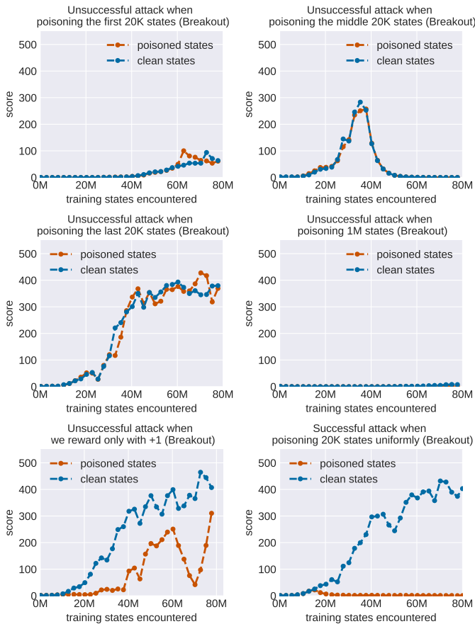
Fig. 1: Attack performances with different manipulation sequences and reward modifications. The first three show the results of poisoning only in the beginning, in the middle and at the end of the training, respectively. The fourth figure presents the case where we poison 1M out of 80M states and the agent fails to learn the task. The last two figures show targeted attacks where we do not set / set the reward to -1 for actions different than the target one, respectively. The last figure shows a successful attack.
